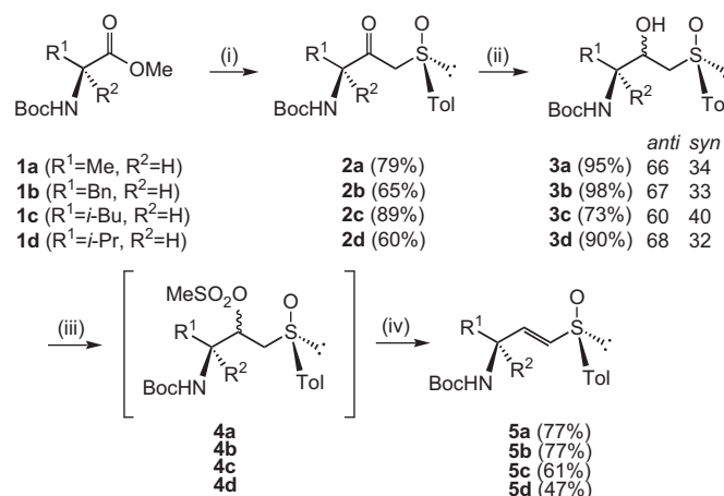
Scheme 1. Reagents and conditions: (i) (+)-( R )- p -TolSOMe, LDA, THF, -78 °C. (ii) NaBH 4 , MeOH, -78 °C. (iii) MeSO 2 Cl, Et 3 N, CH 2 Cl 2 , 25 °C. (iv) t -BuOK, DMSO, 25 °C.
