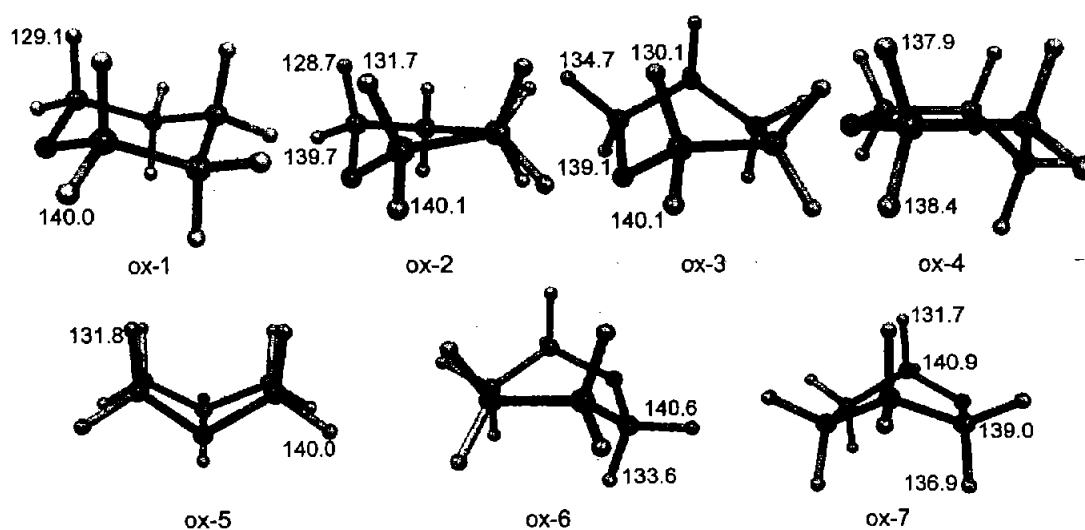
Figure 2. ^1J_{\text{CH}} in the conformations related by inversion of oxane.
