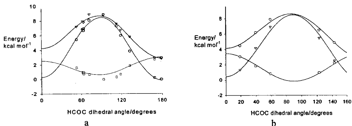
Figure 4. Dependence on dihedral angle of strength of np \rightarrow \sigma^*CH (o), ns \rightarrow \sigma^*CH (•) and ns+np \rightarrow \sigma^*CH^* (∇) delocalizations in a) oxane, b) ethyl methyl ether.
