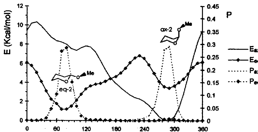
Scheme 6. Energy and population profiles for axial and equatorial 2-OMeTHP as calculated with MM2.
