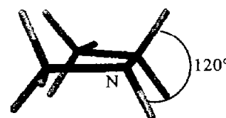
(S)-ema \tau_{HCNC} = 120^\circ
