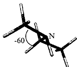
(S)-ema \tau_{HCNC} = -60^\circ
