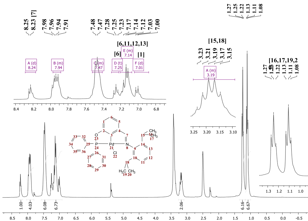
Figura 3.42. Espectro de RMN- ^1\text{H} (300 MHz, \text{CDCl}_3/\text{DMSO}-d_6 ) del paladacilo 3.8 .
