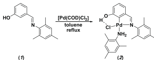
Scheme 2. Synthesis of complex [PdCl(H_2NC_6H_2-2,4,6-Me_3)(C_6H_3-2-(OH)-6-(CH=NC_6H_2-2,4,6-Me_3))] ( 2 ).
