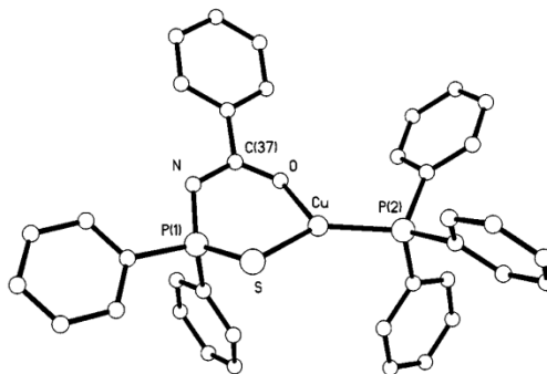
Fig. 2.10: Estructura molecular de [Cu(PPh 3 )(PhC(O)NP(S)Ph 2 )].
