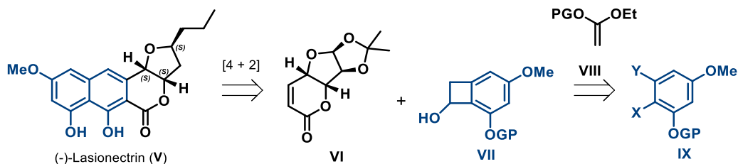
Scheme 2. Proposed retrosynthesis of (-)-Lasionectrine.
